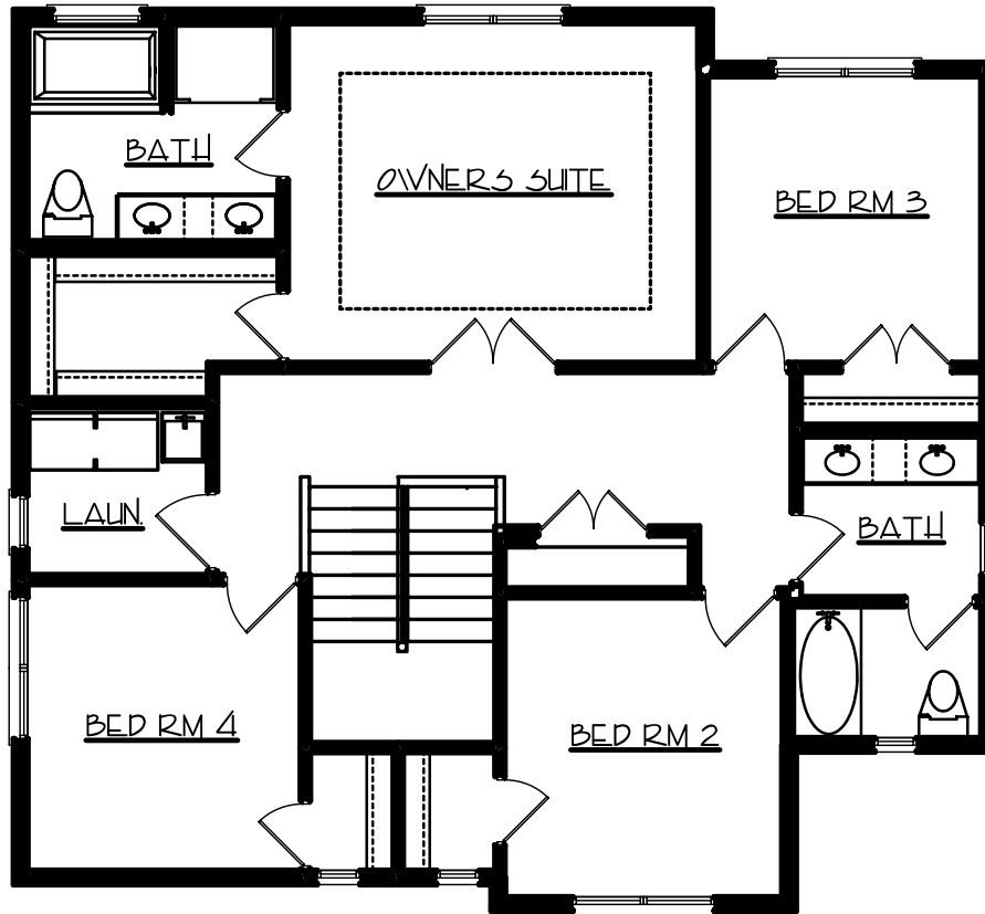
UPPER FLOOR PLAN 1/4" = 1'-0" © COPYRIGHT BEYOND DESIGN ARCHITECTURE
